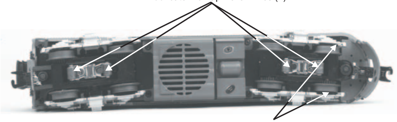
Lubrication Points on the Locomotive Lubricate All Wheel Axles (L)
