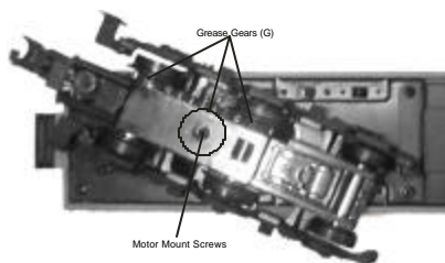
Figure 8: Greasing The Power Trucks
