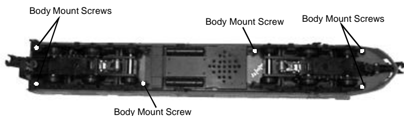
Fig. 9 Removing the body from the chassis
