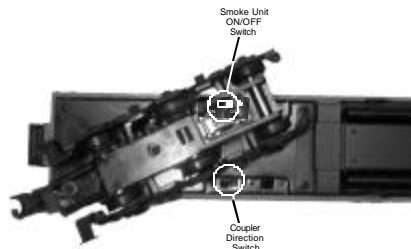
Figure 1b: Locating The Smoke Unit & ProtoCoupler® Selection Switch
