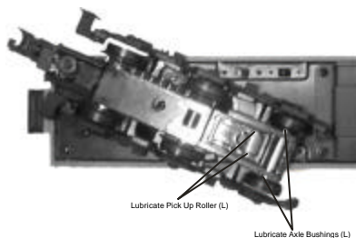
Figure 7: Lubricating The Truck
