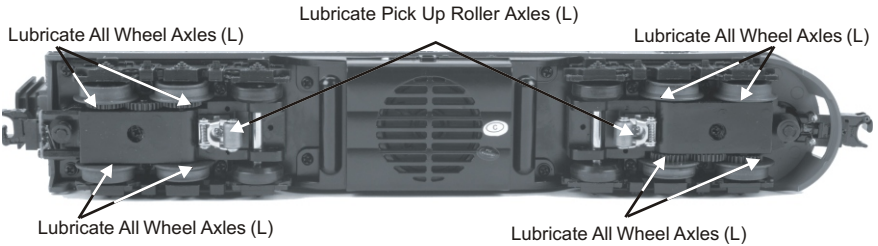
Lubrication Points on the Locomotive
